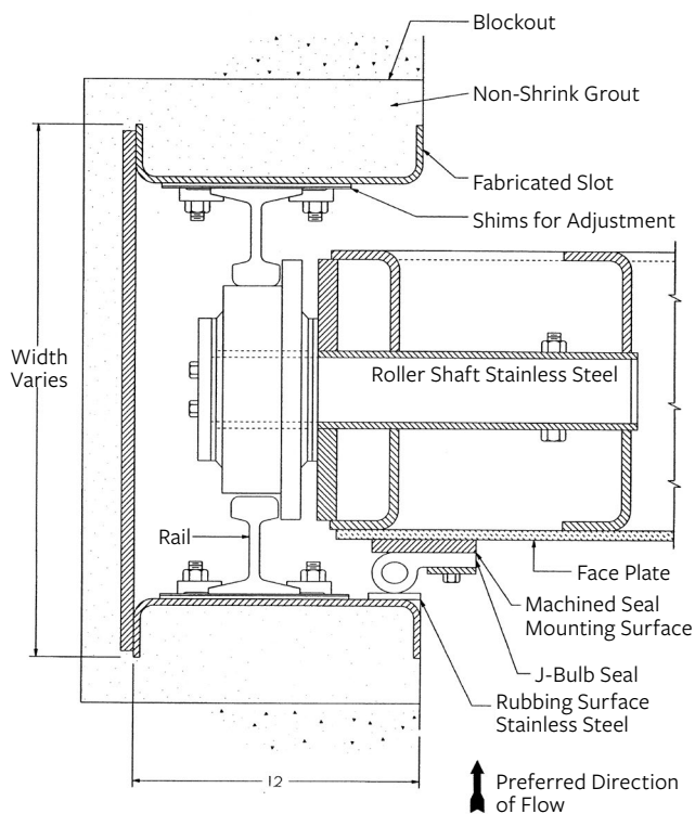
FIGURE 8-1 FABRICATED ROLLER SLOT WITH DOUBLE RAILS
