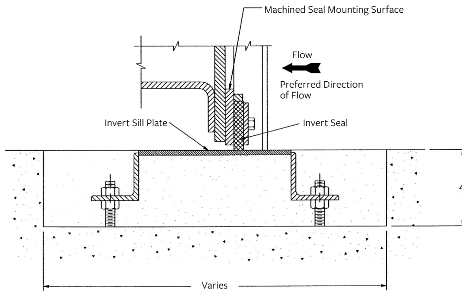
FIGURE 8-3 SILL PLATE DETAIL
