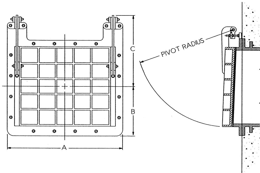
Figure 6-3 Heavy-Duty Flap Gate (Model 50)
