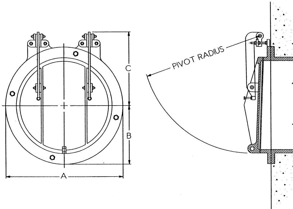
Figure 6-2 Heavy-Duty Flap Gate (Model 50C)
